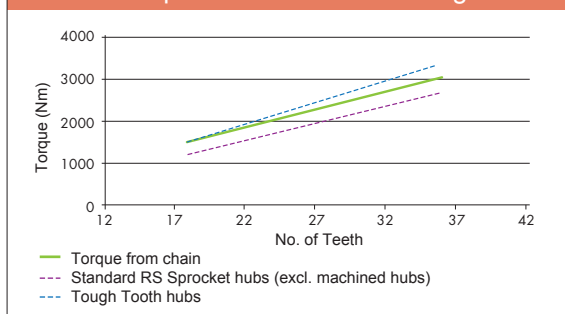
Comparison of Hub kW Ratings
