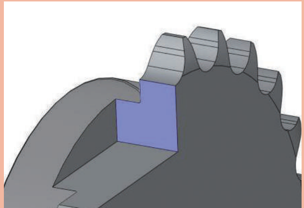
Cross-section observation of tooth hardened layer depth (darker area is the hardened layer)
